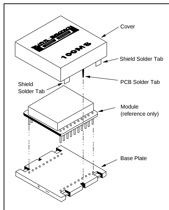
FIGURE 2. Assembly Diagram.
