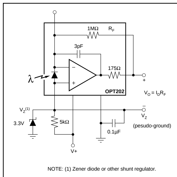
FIGURE 7. Single Power Supply Operation.
