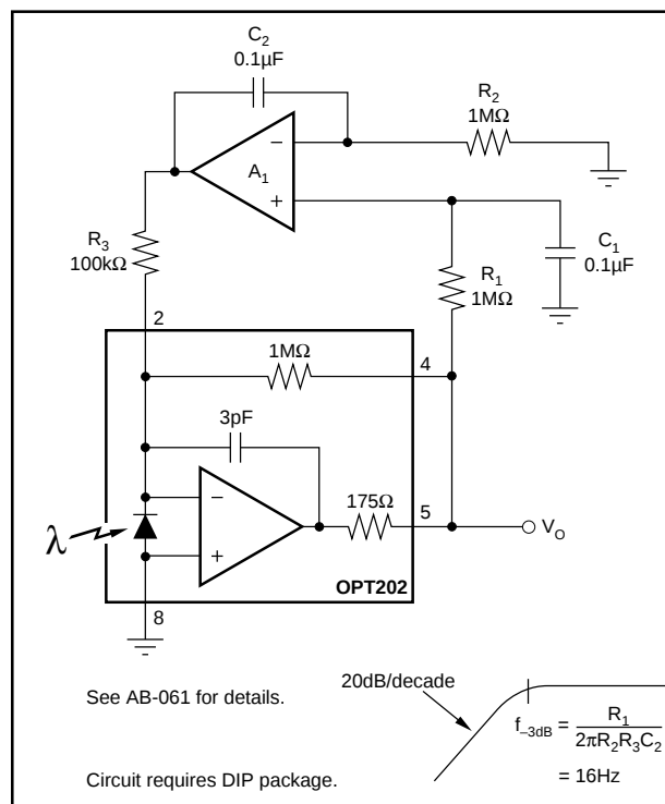
FIGURE 8. DC Restoration Rejects Unwanted Steady-State Background Light.
