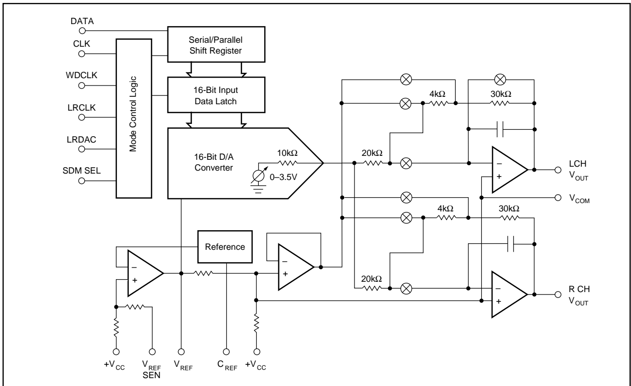
FIGURE 2. PCM66P Block Diagram.
