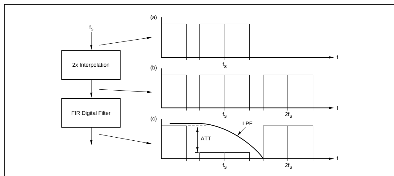
FIGURE 4. Function and Operation of a Digital Filter .
