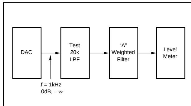
FIGURE 13. SNR (idle channel noise) Test Block Diagram.
