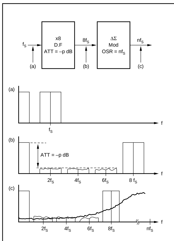
FIGURE 6. Spectrum of a \Delta\Sigma DAC with a Digital Filter.
