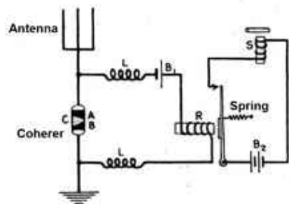
Fig. 101. Marconi 1896 Receiver.
