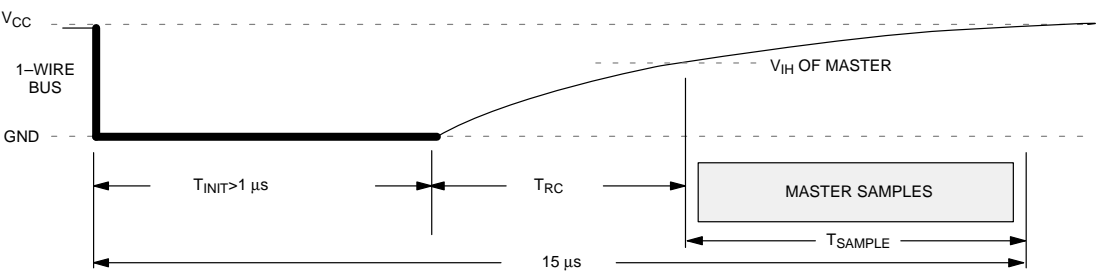
DETAILED MASTER READ ONE TIMING Figure 11
