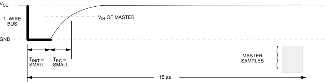
RECOMMENDED MASTER READ ONE TIMING Figure 12
