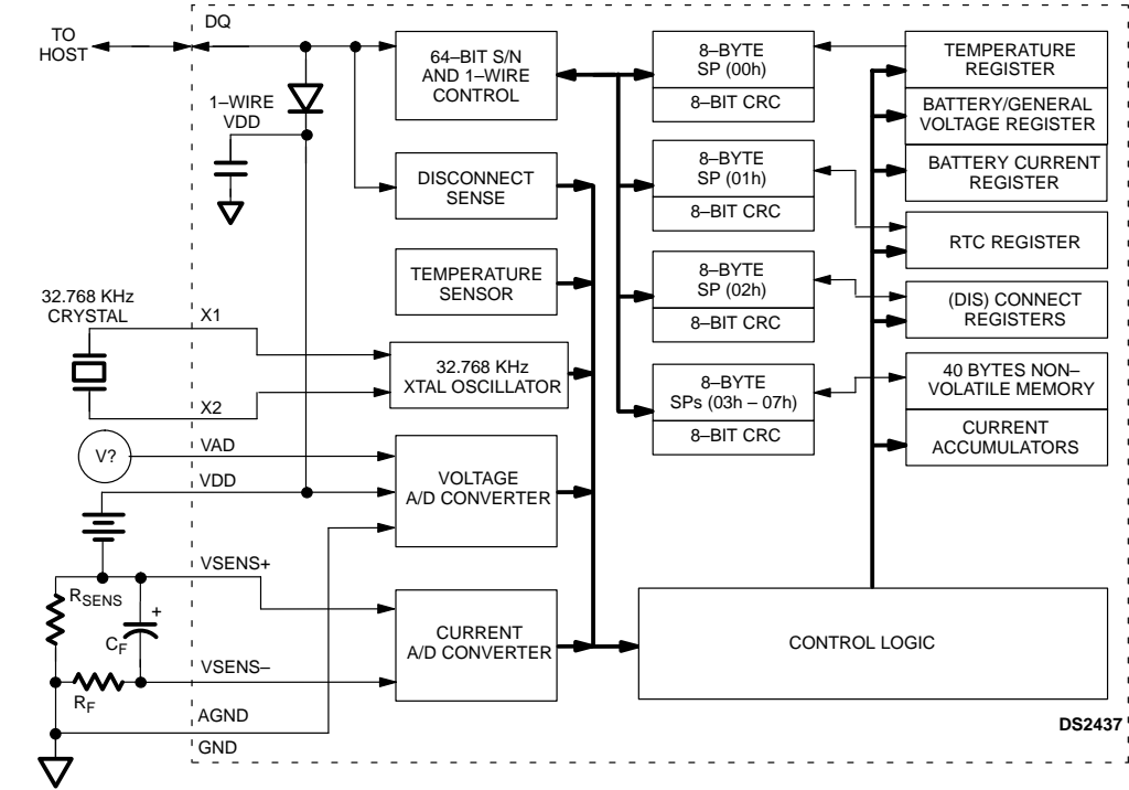
DS2437 BLOCK DIAGRAM Figure 1
