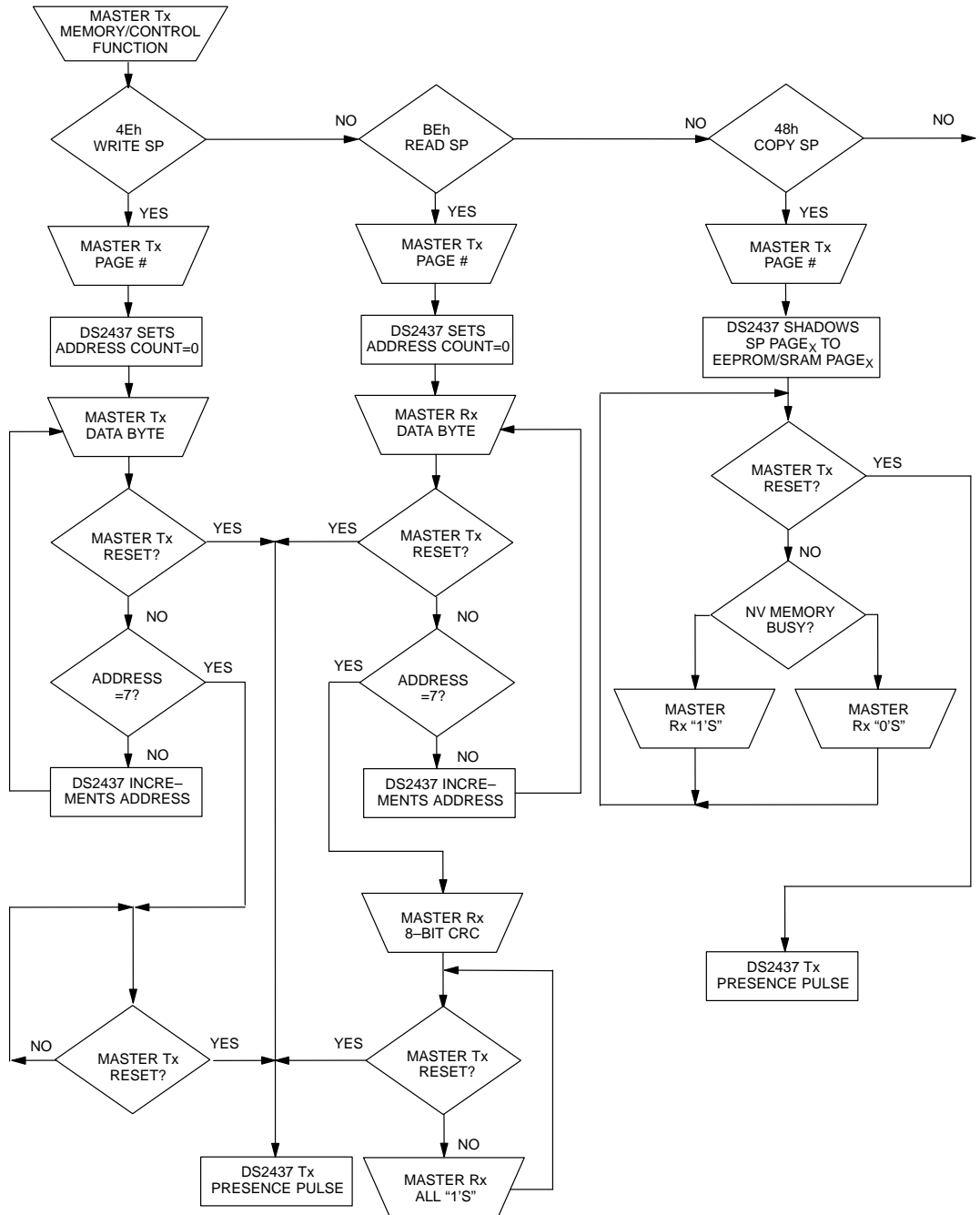
MEMORY/CONTROL FUNCTIONS FLOWCHART Figure 6
