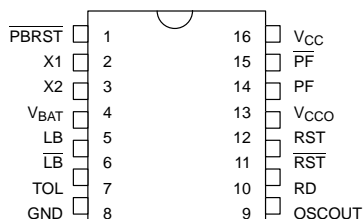
16-Pin DIP (300 Mil) See Mech. Drawings Section
