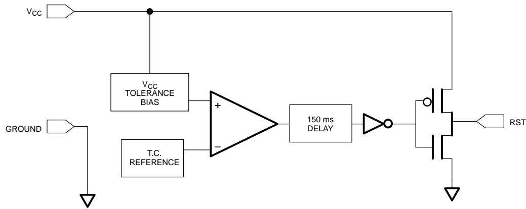
BLOCK DIAGRAM (CMOS OUTPUT) Figure 1
