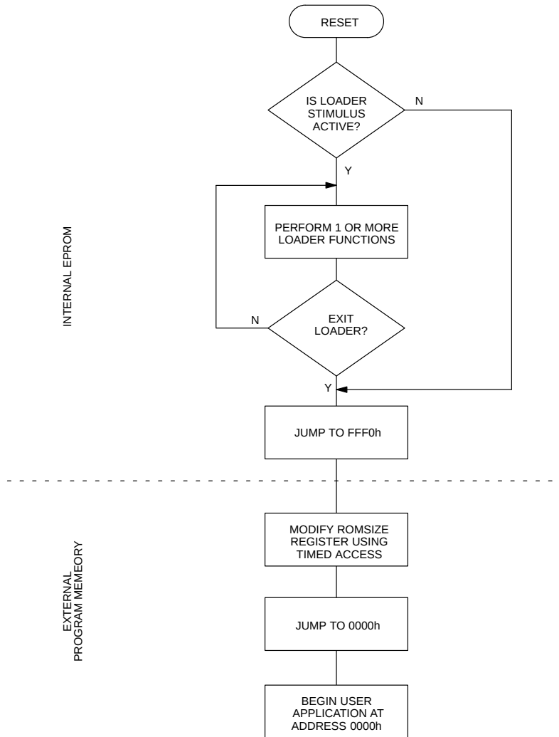
BOOTLOADER FLOWCHART Figure 1
