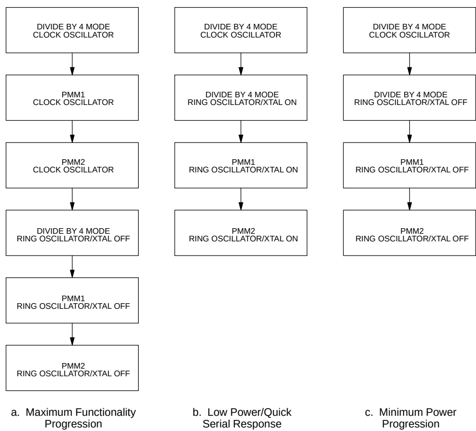
SAMPLE POWER PATHS Figure 8
