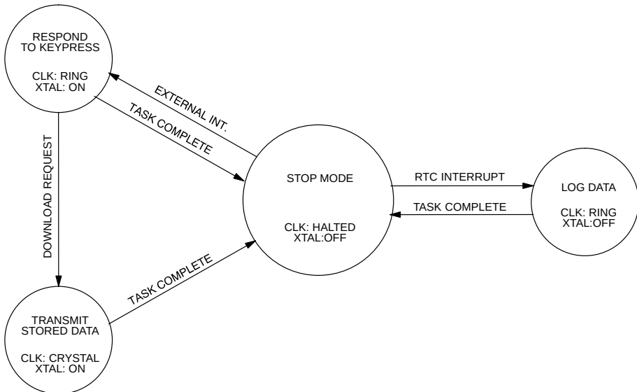
REMOTE DATA LOGGER EXAMPLE STATE DIAGRAM Figure 7
