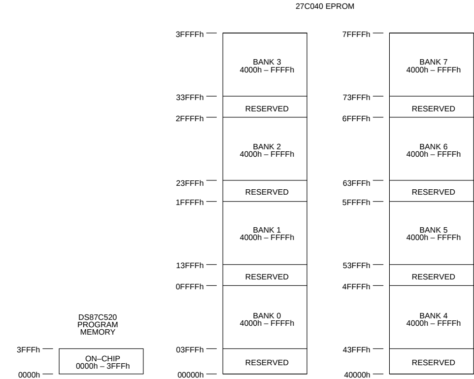
ROMSIZE FEATURE COMMON-PAGE EXPANSION MEMORY MAP Figure 7
