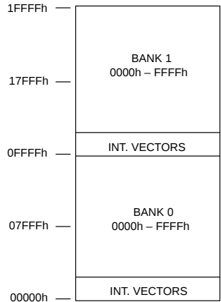
SIMPLE PAGE EXPANSION EXAMPLE MEMORY MAP Figure 2
