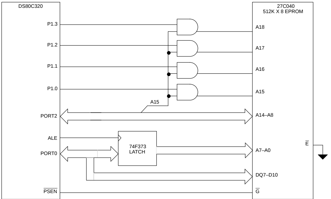
DS80C320 EXPANDED MEMORY EXAMPLE HARDWARE CONFIGURATION Figure 5
