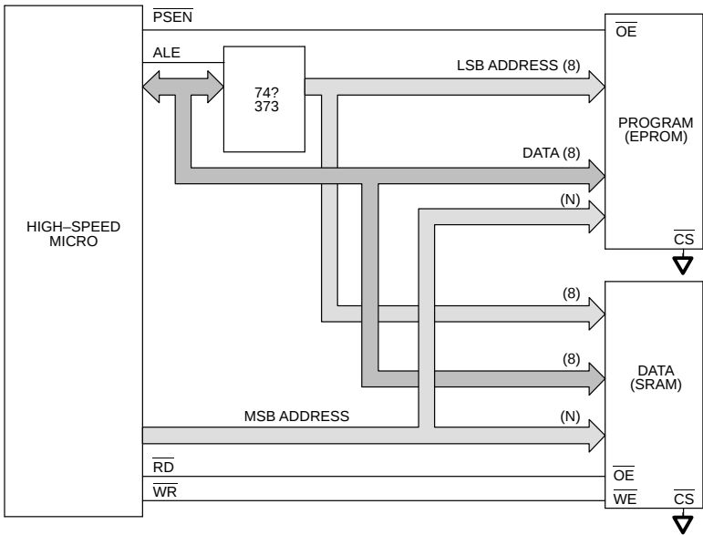
TYPICAL HIGH-SPEED MICRO SYSTEM Figure 1
