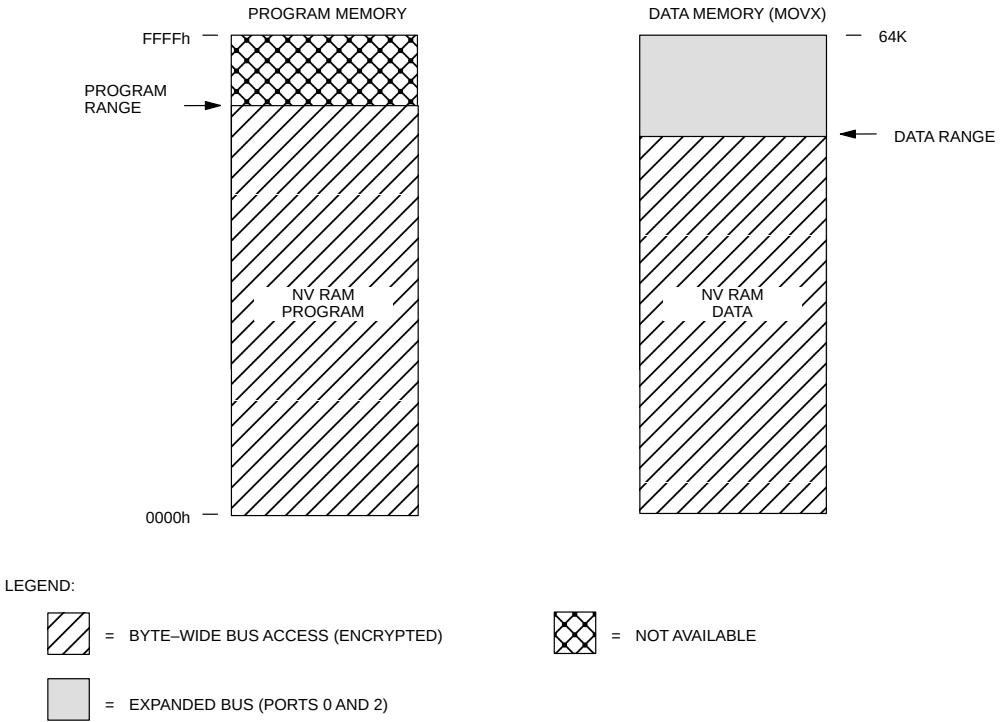
DS5002FP MEMORY MAP IN NON-PARTITIONABLE MODE (PM=1) Figure 3
