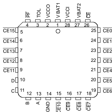
28-Pin PLCC See Mech. Drawings Section
