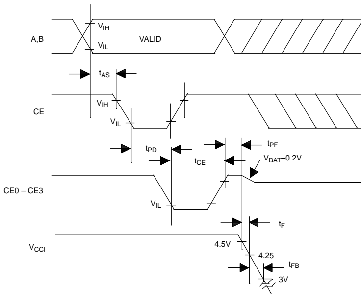
POWER-DOWN Figure 5
