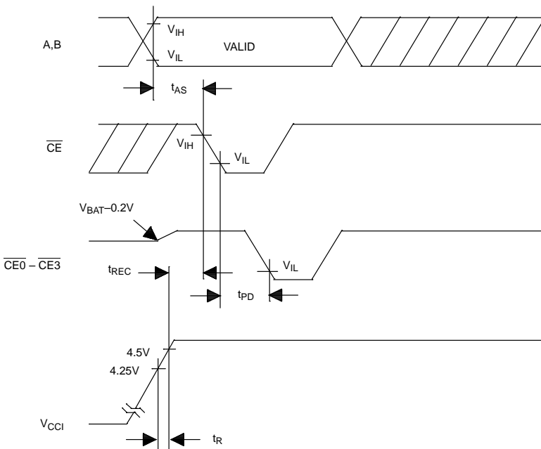
POWER-UP Figure 6
