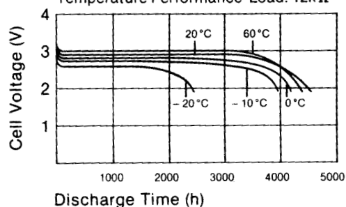
Temperature Performance Load: 12kΩ
