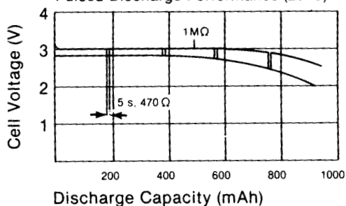
Pulsed Discharge Performance (20°C)
