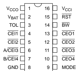
DS1321 16-PIN DIP (300 MIL)
