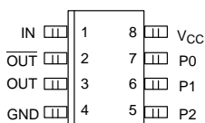
DS1040Z 8-PIN SOIC (150 MIL) See Mech. Drawings Section
