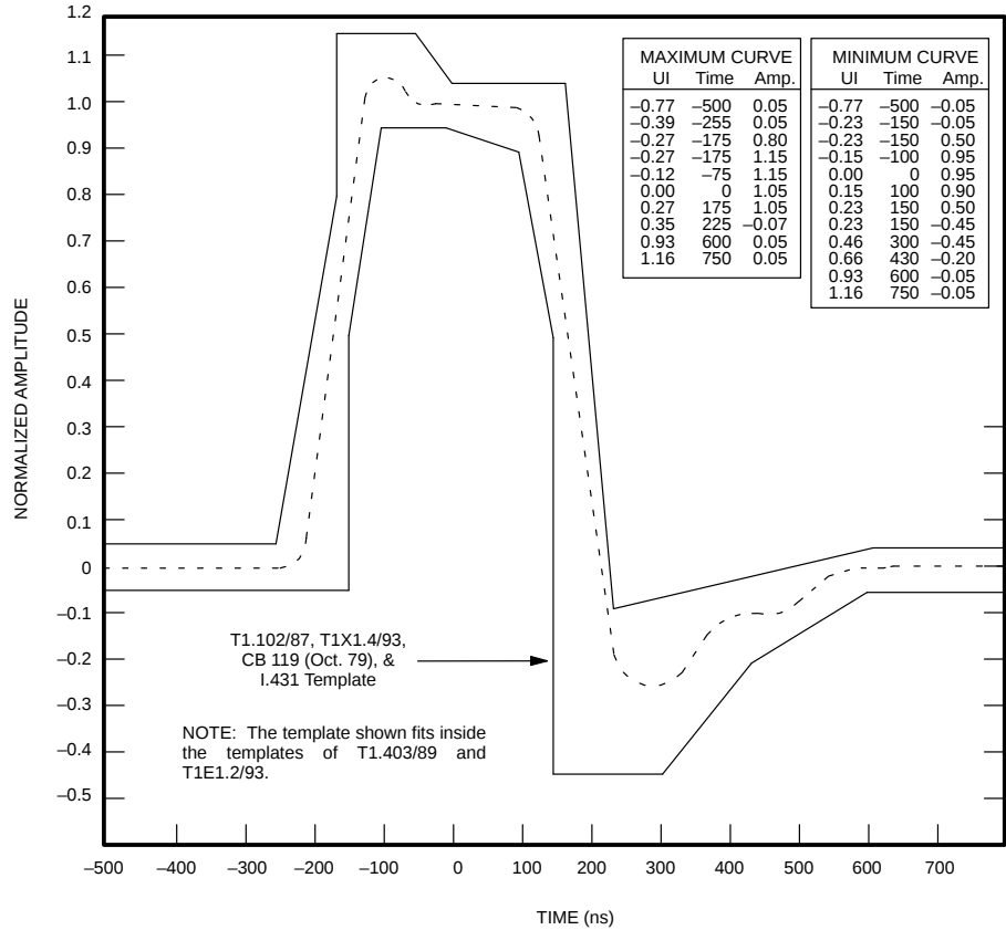
DS2151Q TRANSMIT WAVEFORM TEMPLATE Figure 12–3
