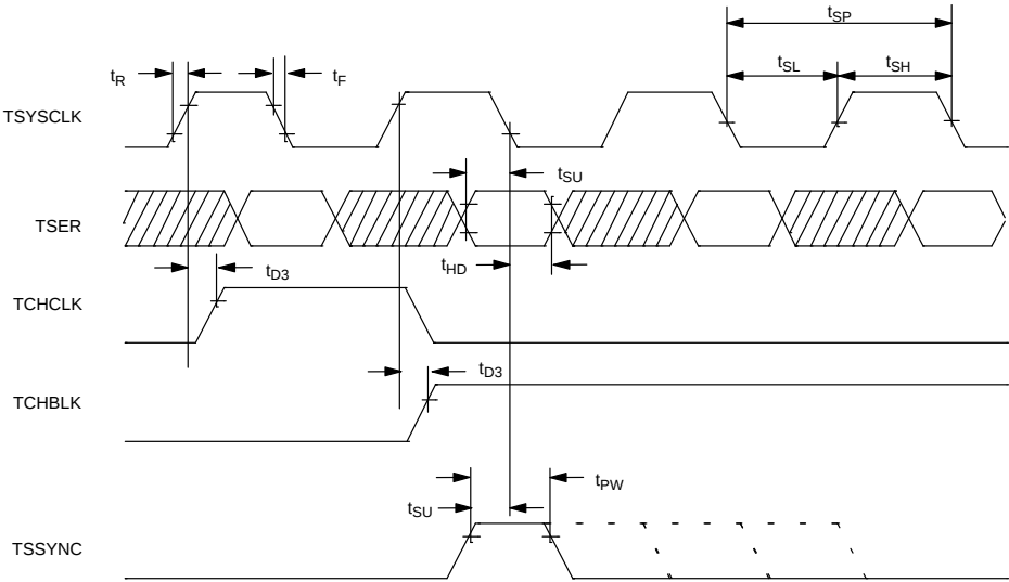
TRANSMIT SYSTEM SIDE AC TIMING Figure 16–8
