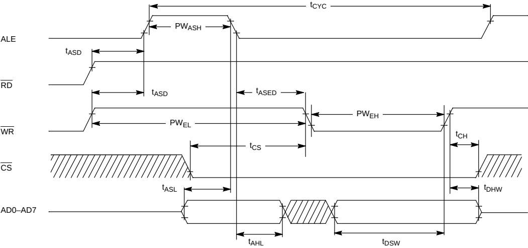
INTEL BUS WRITE AC TIMING (BTS=0/MUX=1) Figure 16–2
