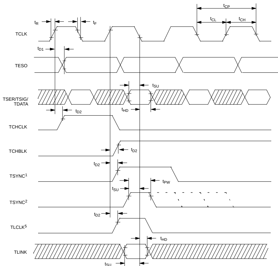
TRANSMIT SIDE AC TIMING Figure 16–7
