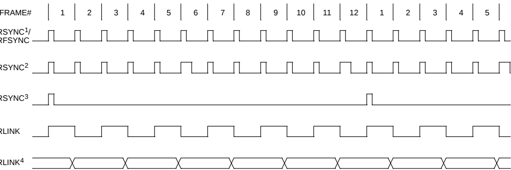
RECEIVE SIDE D4 TIMING Figure 15–1
