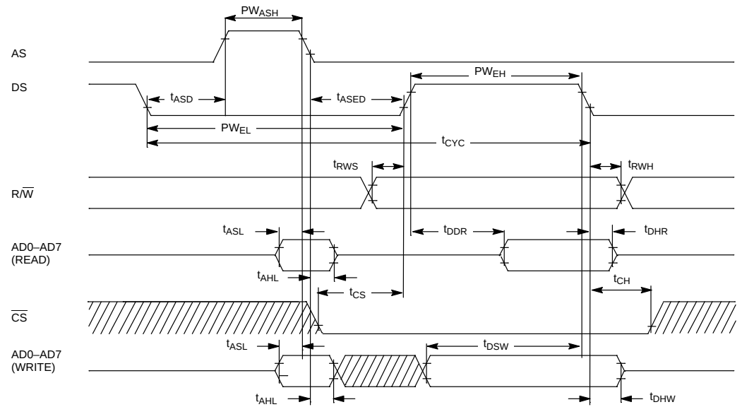
MOTOROLA BUS AC TIMING (BTS=1/MUX=1) Figure 16–3
