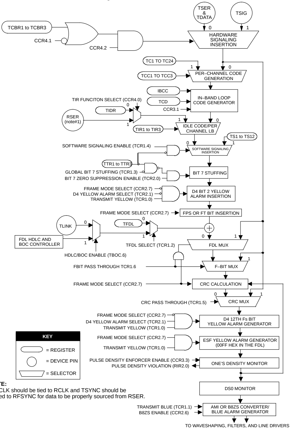
DS2152 TRANSMIT DATA FLOW Figure 15–11
