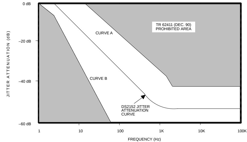
DS2152 JITTER ATTENUATION Figure 14–4
