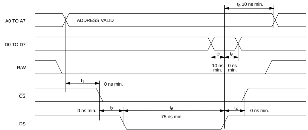
MOTOROLA BUS WRITE AC TIMING (BTS=1/MUX=0) Figure 16-13
