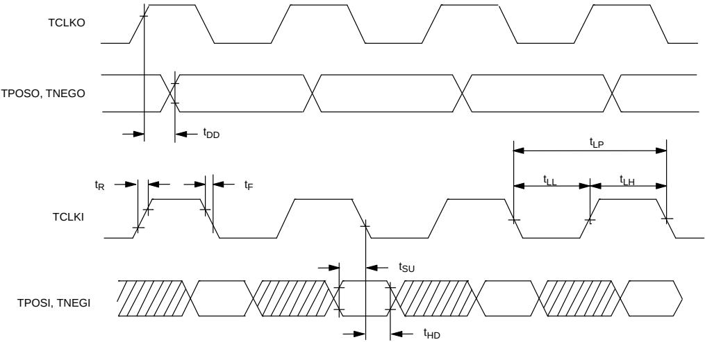
TRANSMIT LINE INTERFACE SIDE AC TIMING Figure 16–9
