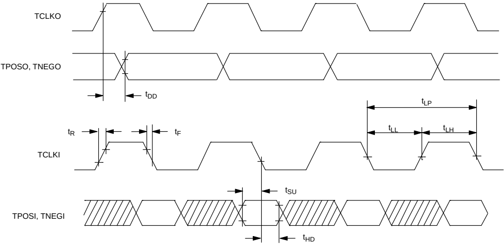
TRANSMIT LINE INTERFACE SIDE AC TIMING Figure 14–9
