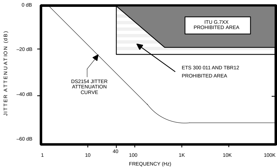
DS2154 JITTER ATTENUATION Figure 12-4
