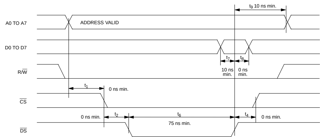
MOTOROLA BUS WRITE AC TIMING (BTS=1/MUX=0) Figure 14–13
