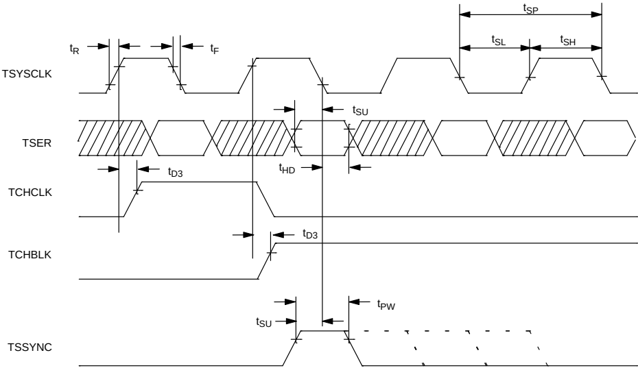
TRANSMIT SYSTEM SIDE AC TIMING Figure 14–8
