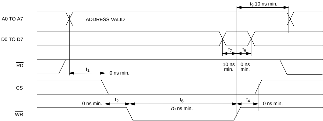
MOTOROLA BUS READ AC TIMING (BTS=1/MUX=0) Figure 14–12
