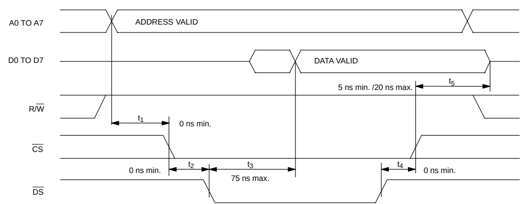
MOTOROLA BUS WRITE AC TIMING (BTS=1/MUX=0) Figure 14–13
