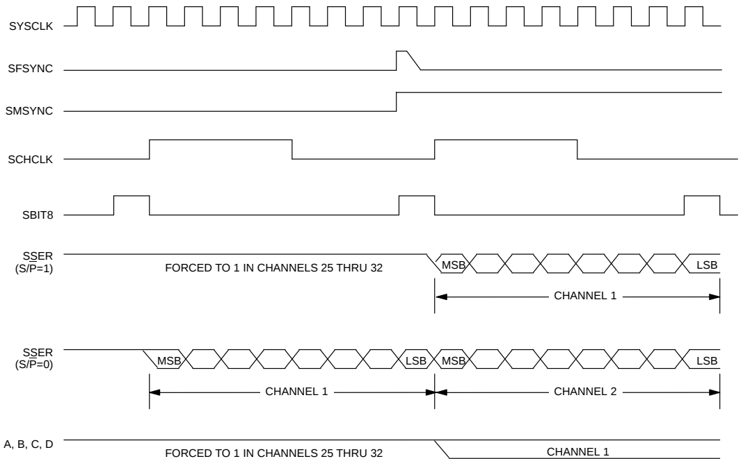
SYSTEM MULTIFRAME BOUNDARY TIMING (SYSCLK = 2.048 MHz) Figure 4
