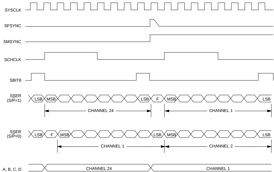
SYSTEM MULTIFRAME BOUNDARY TIMING (SYSCLK = 1.544 MHz) Figure 3
