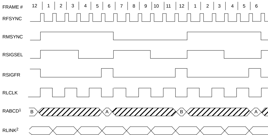
193S RECEIVE MULTIFRAME TIMING Figure 14
