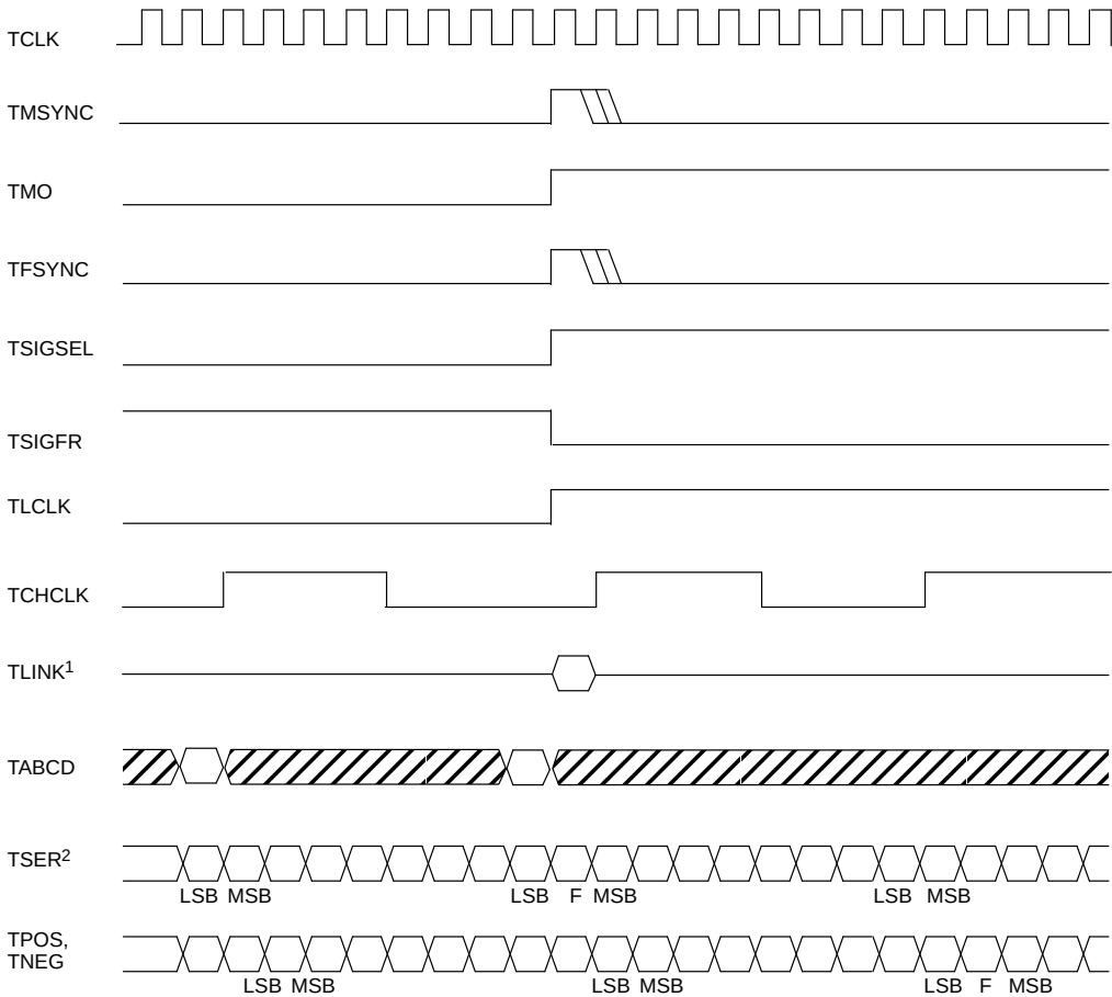
TRANSMIT MULTIFRAME BOUNDARY TIMING Figure 11
