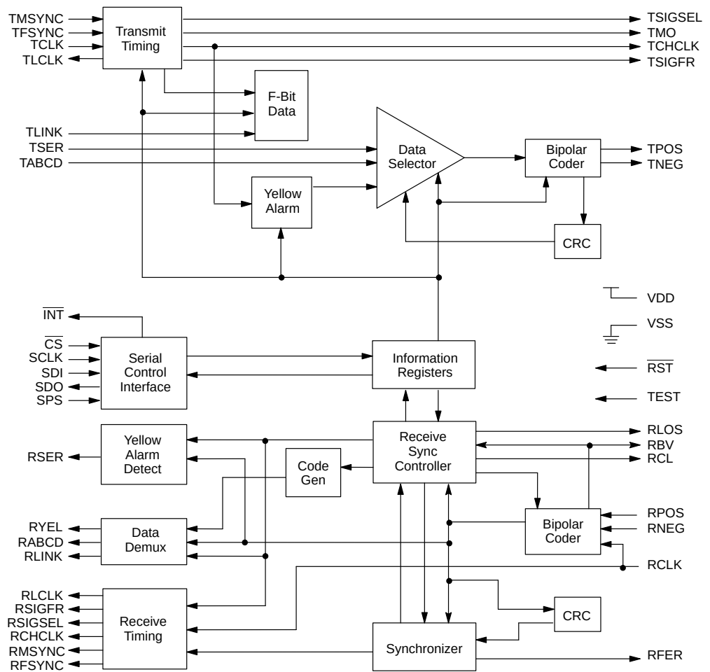
DS2180A BLOCK DIAGRAM Figure 1
