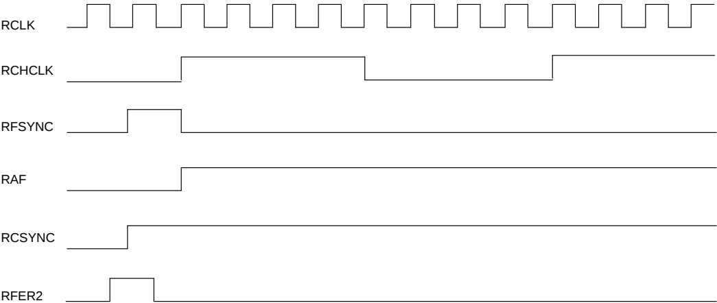
CRC4 SUB-MULTIFRAME 2 ERRORED Figure 25
