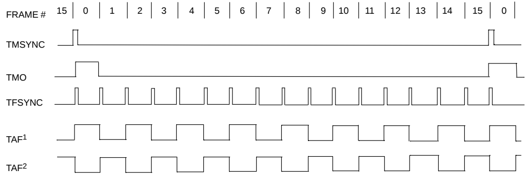
TRANSMIT MULTIFRAME TIMING Figure 12
