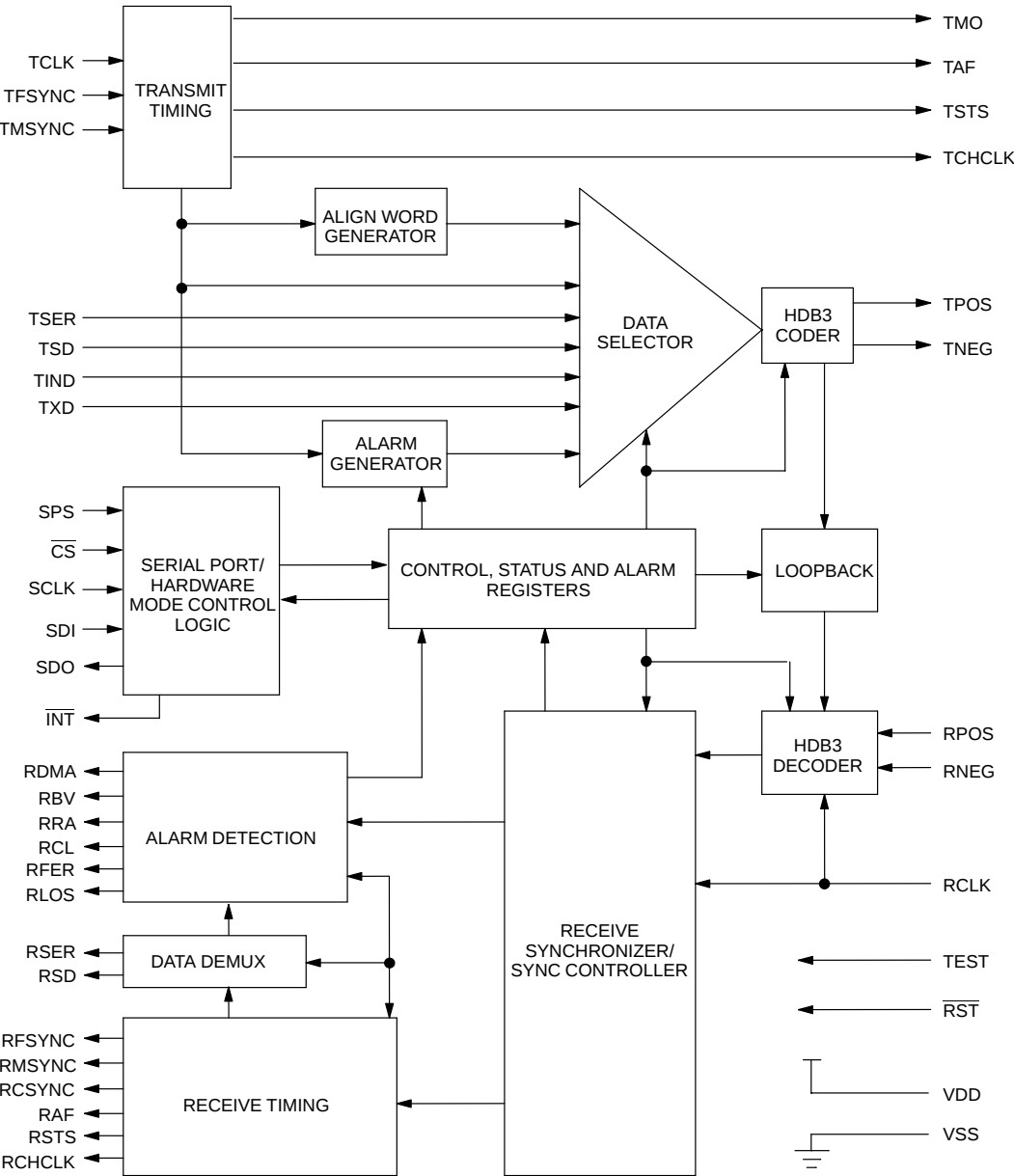
DS2181A BLOCK DIAGRAM Figure 1
