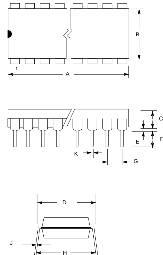
DS2187 RECEIVE LINE INTERFACE 18-PIN DIP
