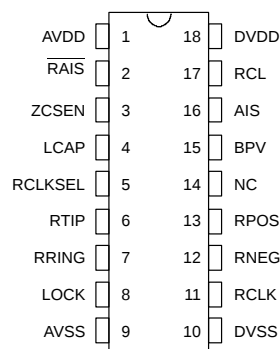
18-Pin DIP (300 Mil)
