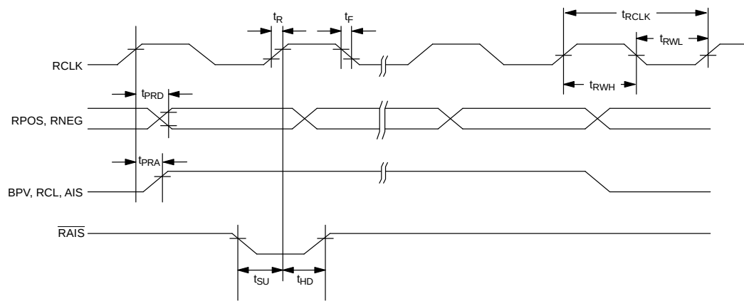
AC TIMING DIAGRAM Figure 4
