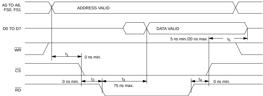
INTEL BUS READ AC TIMING (BTS=0/MUX=0) Figure 12–10
