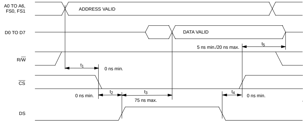
MOTOROLA BUS READ AC TIMING (BTS=1/MUX=0) Figure 12-12
