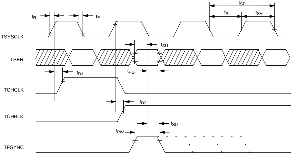
TRANSMIT SYSTEM SIDE AC TIMING Figure 12–9
