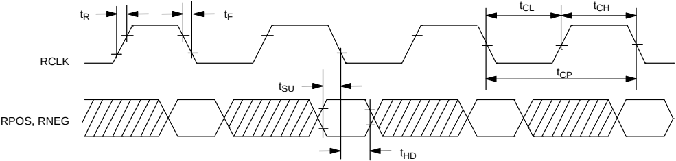
RECEIVE LINE INTERFACE AC TIMING Figure 12–6
