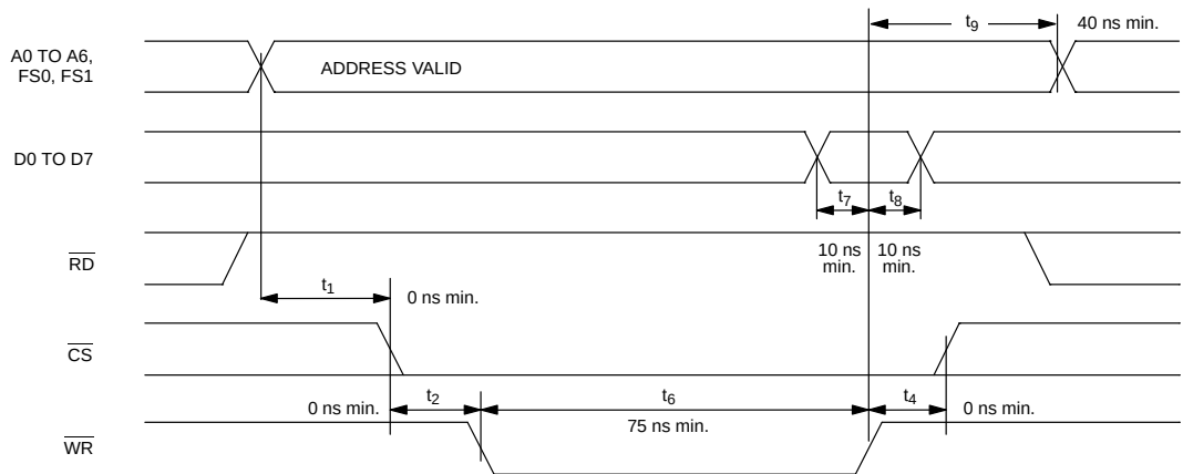
INTEL BUS WRITE AC TIMING (BTS=0/MUX=0) Figure 12–11
