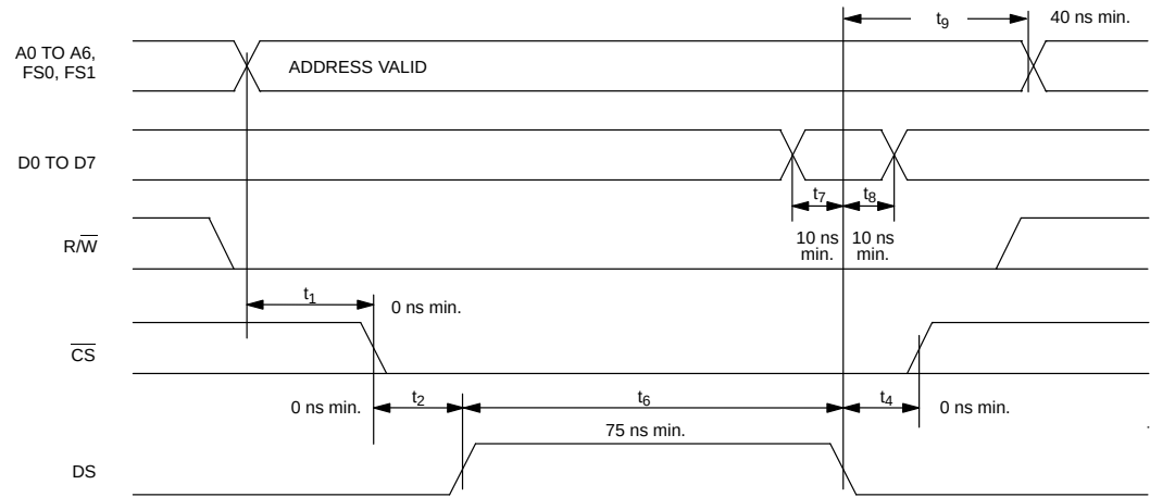
MOTOROLA BUS WRITE AC TIMING (BTS=1/MUX=0) Figure 12-13
