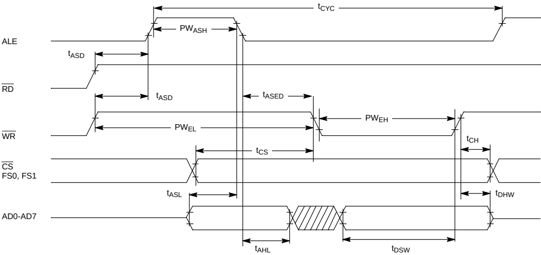
INTEL BUS WRITE AC TIMING (BTS=0/MUX=1) Figure 12–2
