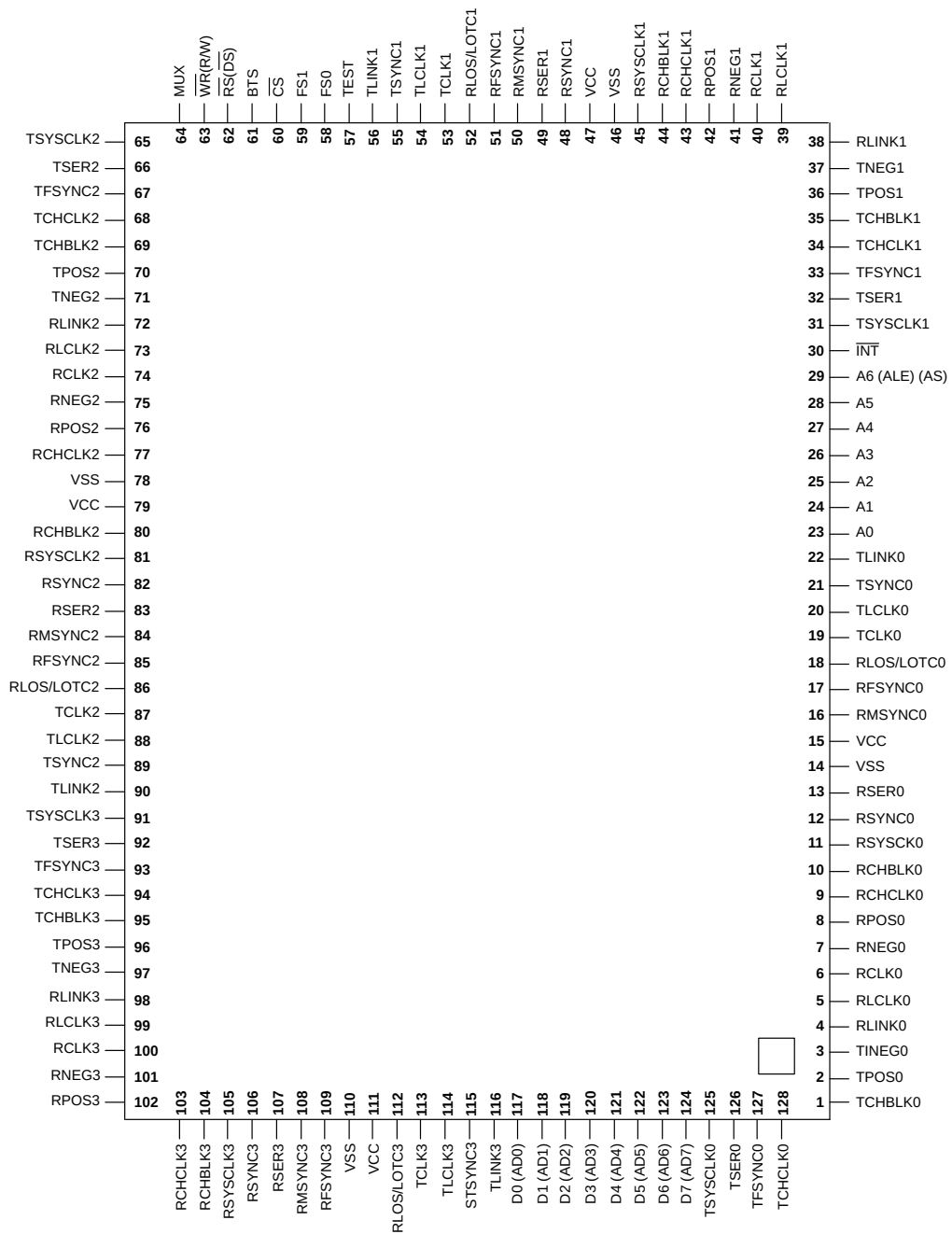
PIN-OUT CONFIGURATION Figure 1–2
