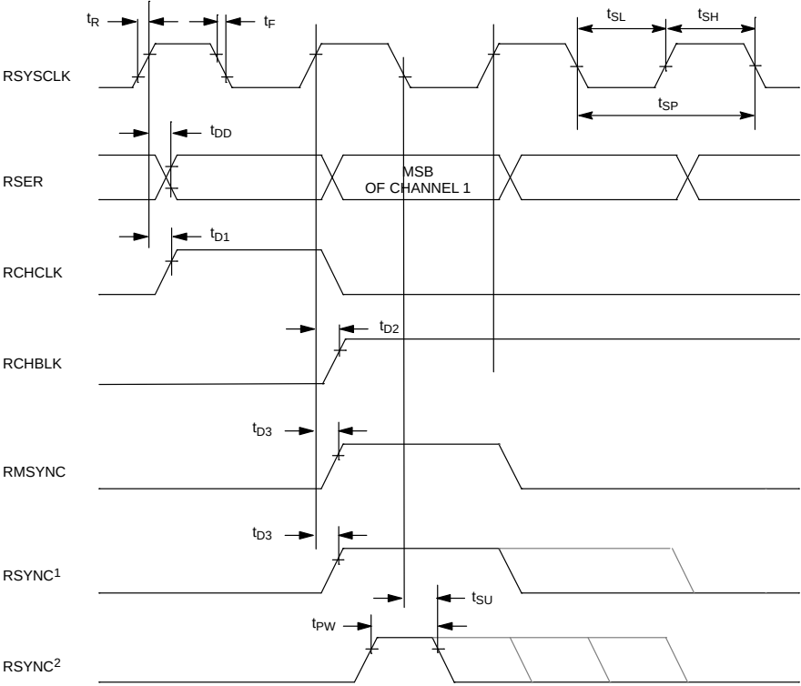
RECEIVE SYSTEM SIDE AC TIMING Figure 12–5
