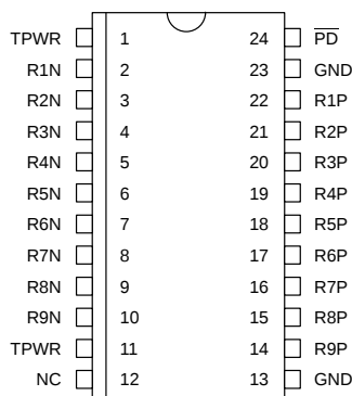
DS2108S 24-PIN SOIC (300 MIL)
