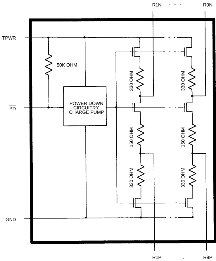
DS2108 BLOCK DIAGRAM Figure 1
