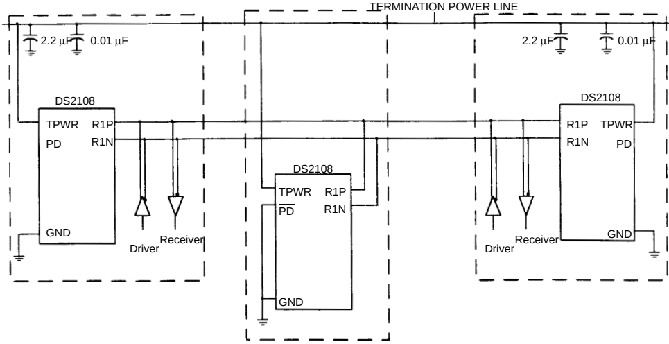
TYPICAL DIFFERENTIAL SCSI BUS CONFIGURATION Figure 2
