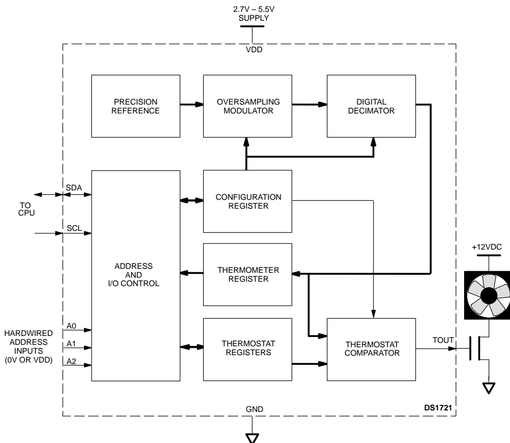
DS1721 FUNCTIONAL BLOCK DIAGRAM Figure 1
