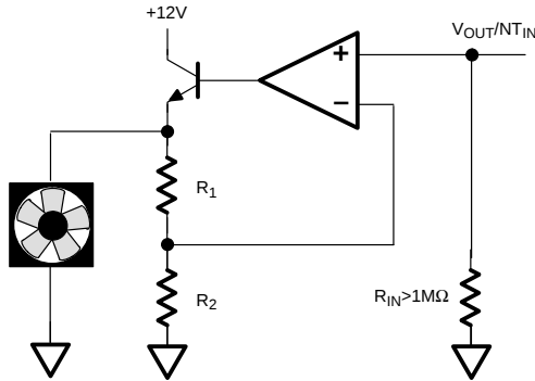
FAN AMPLIFIER CIRCUIT EXAMPLE Figure 6
