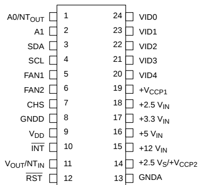
DS1780E 24-PIN TSSOP (173 MIL)
