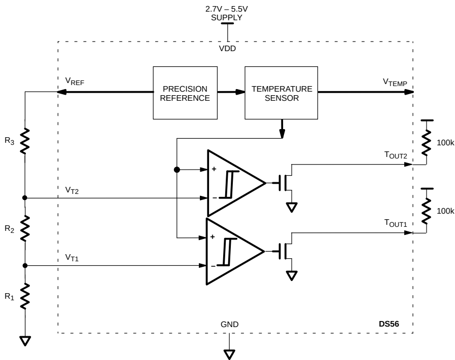
DS56 FUNCTIONAL BLOCK DIAGRAM Figure 1
