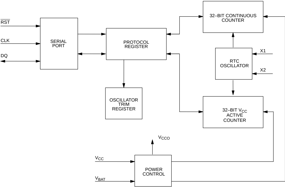
DS1602 ELAPSED TIME COUNTER BLOCK DIAGRAM Figure 1
