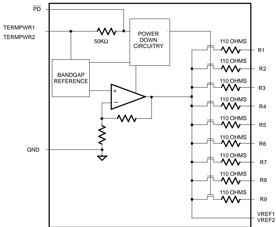
DS21T07 BLOCK DIAGRAM Figure 1
