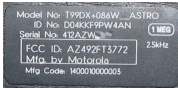
Figure 5.2 A photo illustration of a model number tag on the rear of a Motorola Inc. ASTRO Digital Spectra™. There are several useful pieces of information displayed in the tag, including the model number, serial number, manufacture code (FLASHport™), host firmware flash ROM size (1M) and indication of a 2.5 KHz narrow-band RF board.
