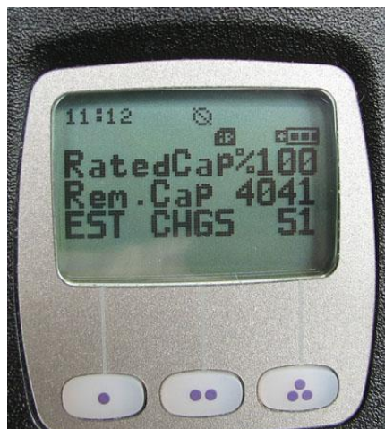
Figure 6.6 A photo illustration of a Motorola XTS 5000™ displaying IMPRES™ battery data via the BATT soft-menu. In addition to this data, note the battery gauge in the upper-right display.
