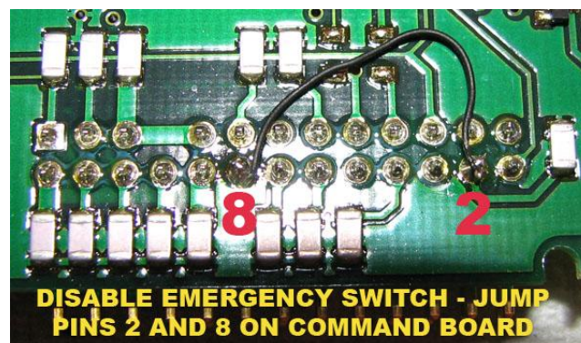
Figure 5.5 A photo illustration showing pins 2 and 8 jumpered on the ASTRO Digital Spectra™ command board. This completes the normally-closed emergency button switch, and prevents it from becoming activated. The radio behaves erratically when this switch is left open.
