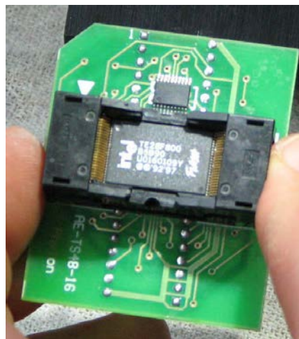
Figure 11.3 A flash ROM from an ASTRO Digital Spectra™ is shown seated in a TSOP-48 adapter in preparation for a firmware upgrade. The firmware write-time to the chip is typically less than one minute.
