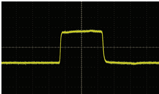
20 ns pulse envelope at 10 GHz RF
