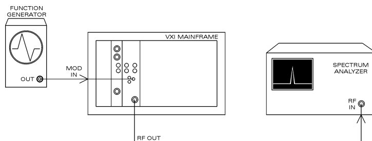
Figure 4-6: Pulse Modulation On/Off Ratio Test
