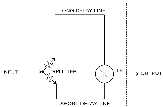
Figure 4-11: FM Test Fixture
