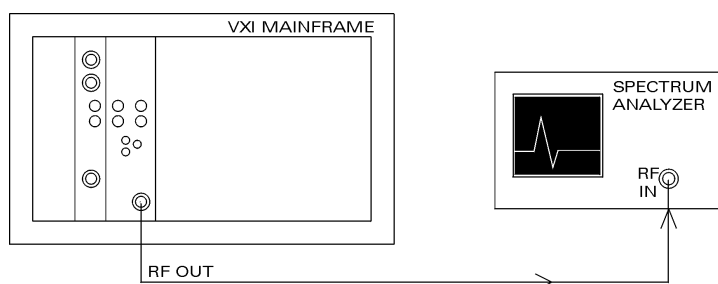
Figure 4-3: Spurious Signals Tests
