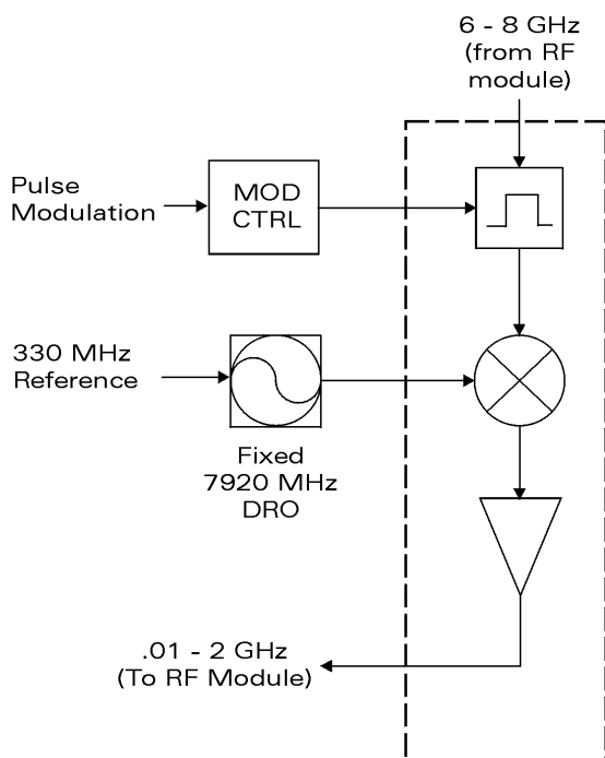
Figure 3-11: Downconverter Circuit
