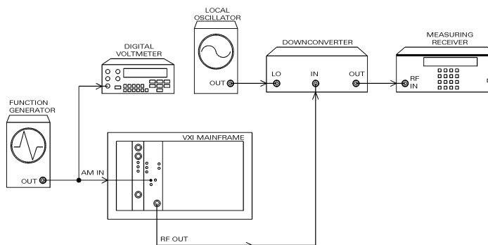
Figure 4-9: Amplitude Modulation Tests
