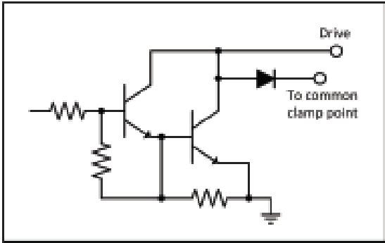
Typical Darlington Channel (1 of 32)
