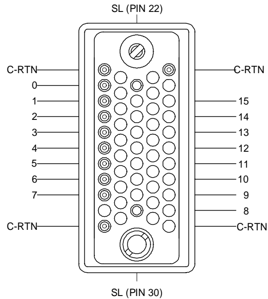
51 pin REDEL HV connector
