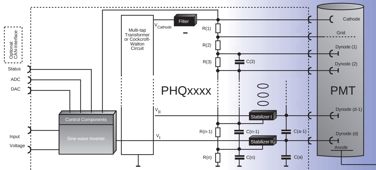
Block Diagram of PHQxxxx
