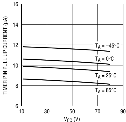
TIMER Pin Pull Up Current vs V_{\text{CC}}
