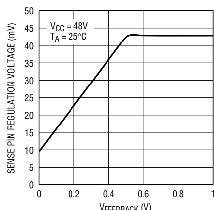
SENSE Pin Regulation Voltage vs V_{\text{FEEDBACK}}
