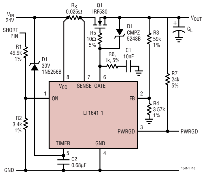
Figure 10. Overvoltage Detection
