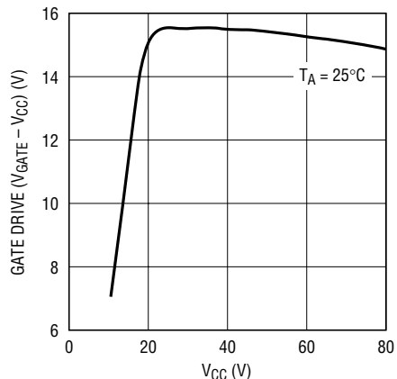
Gate Drive vs V_{\text{CC}}
