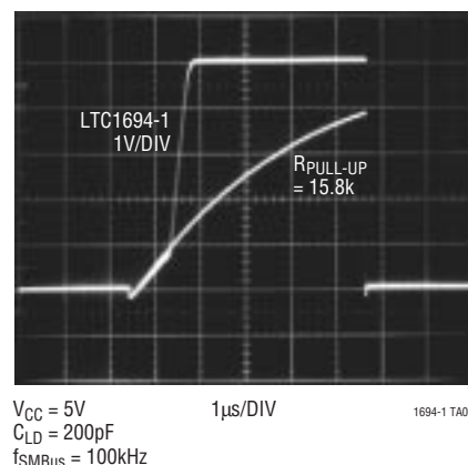
Comparison of SMBus Waveforms for the LTC1694-1 vs Resistor Pull-Up
