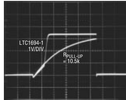
Comparison of SMBus Waveforms for the LTC1694-1 vs Resistor Pull-Up
