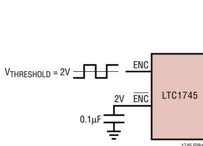
Figure 8a. Single-Ended \overline{\text{ENC}} Drive, Not Recommended for Low Jitter
