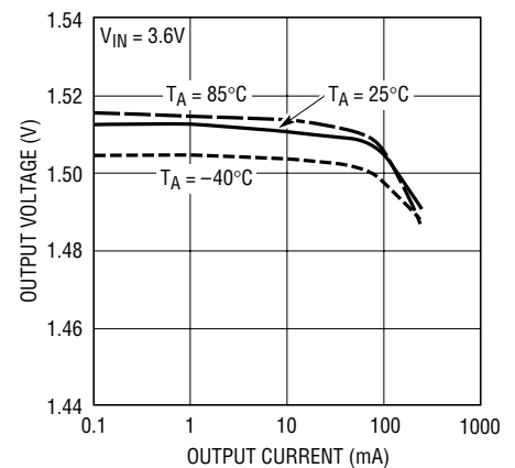
LTC1911-1.5 Output Voltage vs Output Current
