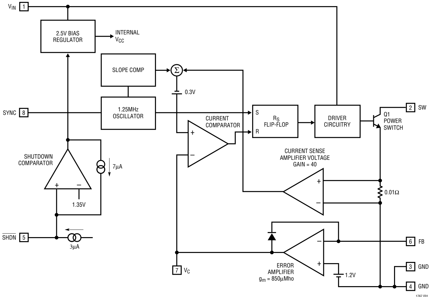
Figure 1. Block Diagram
