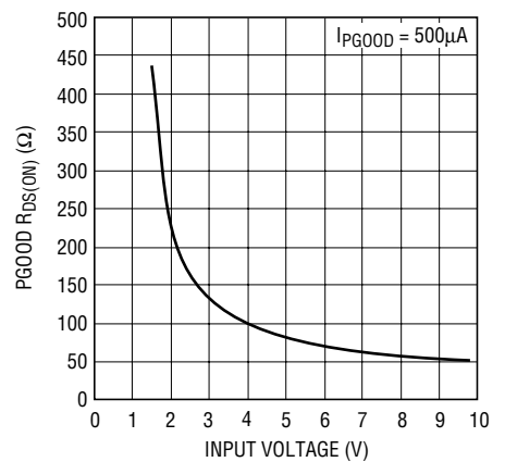
PGOOD RON vs Input Voltage
