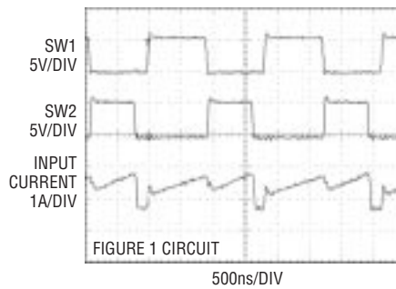
2-Phase Operation
