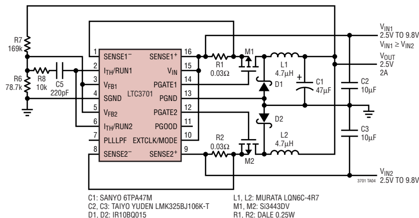
2-Phase, 550kHz, Dual Input Voltage Single Output Step-Down DC/DC Converter
