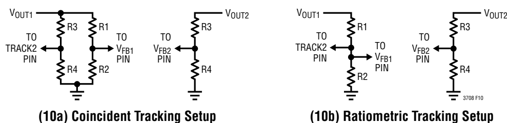
Figure 10. Setup for Coincident and Ratiometric Tracking
