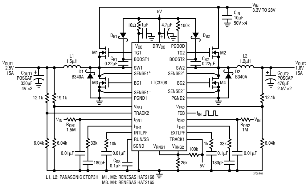
Figure 1. High Efficiency Dual Output Step-Down Converter
