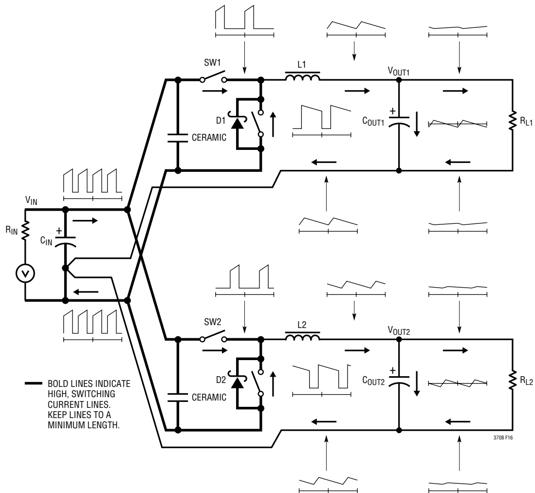
Figure 16. Branch Current Waveforms
