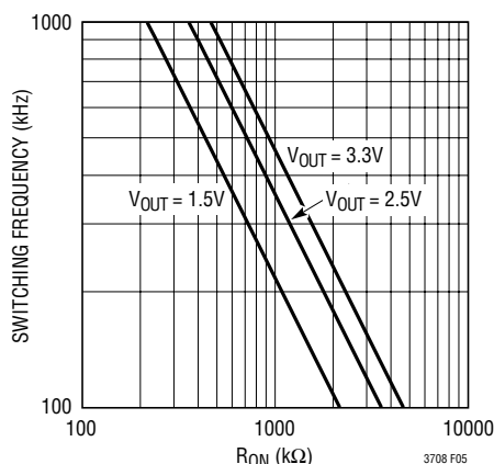
Figure 5. Switching Frequency vs R_{ON}
