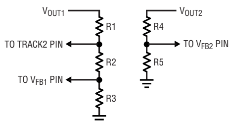
Figure 12. Alternative Setup for Coincident Tracking
