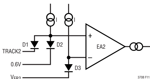
Figure 11. Equivalent Input Circuit of Error Amplifier of Channel 2
