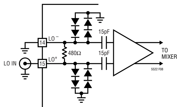
Figure 8. LO Input Schematic
