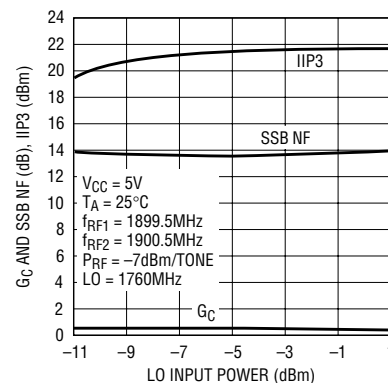
Conv Gain, IIP3 and SSB NF vs LO Power (1.9GHz)
