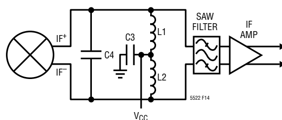
Figure 14. Bandpass IF Matching for Differential IF Architectures
