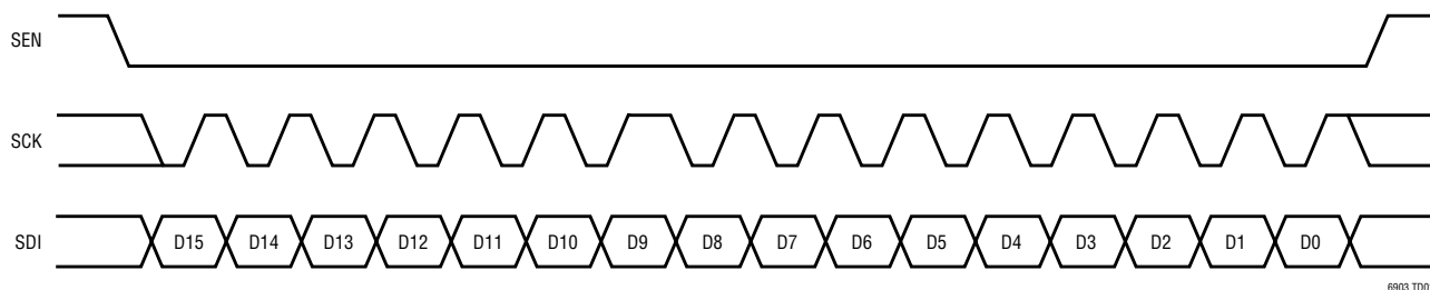
Timing Diagram (LTC6903)
