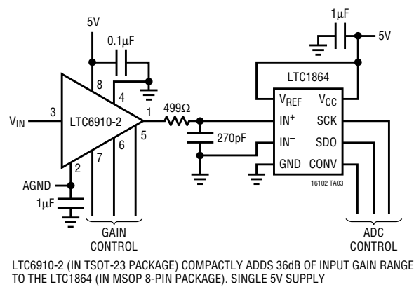
Expanding an ADC's Dynamic Range
