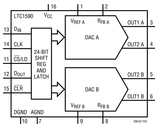
Figure 1. This Single-Supply, Dual 12-Bit DAC Features Serial Interface, \pm 10 V Reference Input Range and a CLR Pin That Resets the Output to Zero
