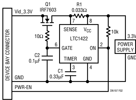
Figure 2. Vid_3.3V Supply Solution for DB32, DB20 and DB13 Form Factors
