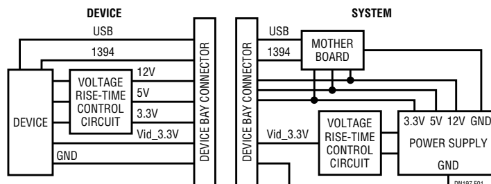
Figure 1. Block Diagram for the Device Bay
