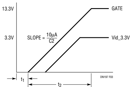
Figure 3. Supply Turn On
