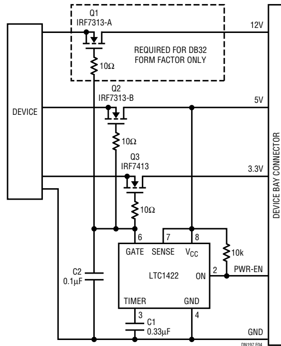
Figure 4. Device Side Voltage Ramp-Up Circuit for DB32, DB20 and DB13 Form Factors
